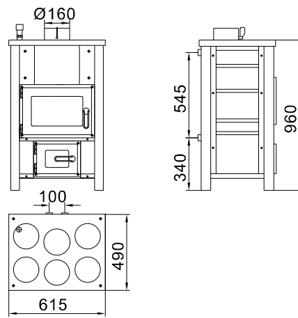
BETI CENTRAL 28kW
