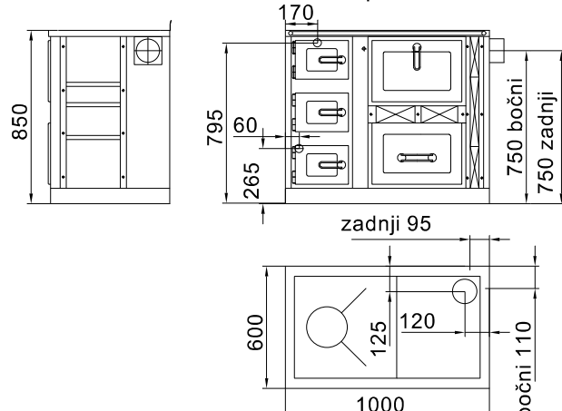
BETI CENTRAL 28kW
